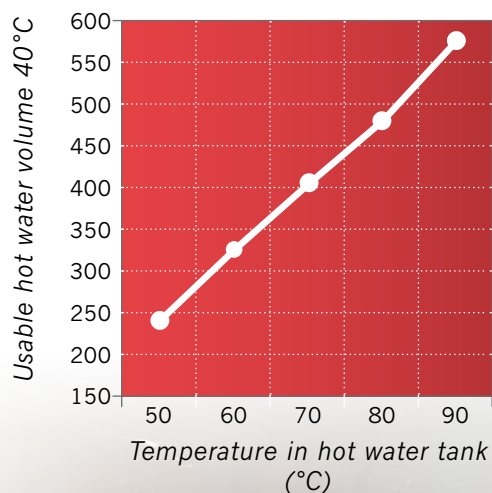
Availability of usable hot water (40°C) in 180 liters hot water tank with HGW technology
